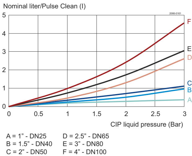
Figure 2. Unique SSV valves 1" DN25 to 4" DN100 Air pressure 6 bar
