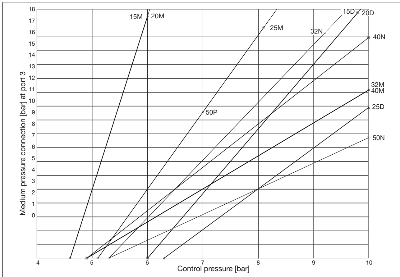
Fig. 3: Control pressure diagram
