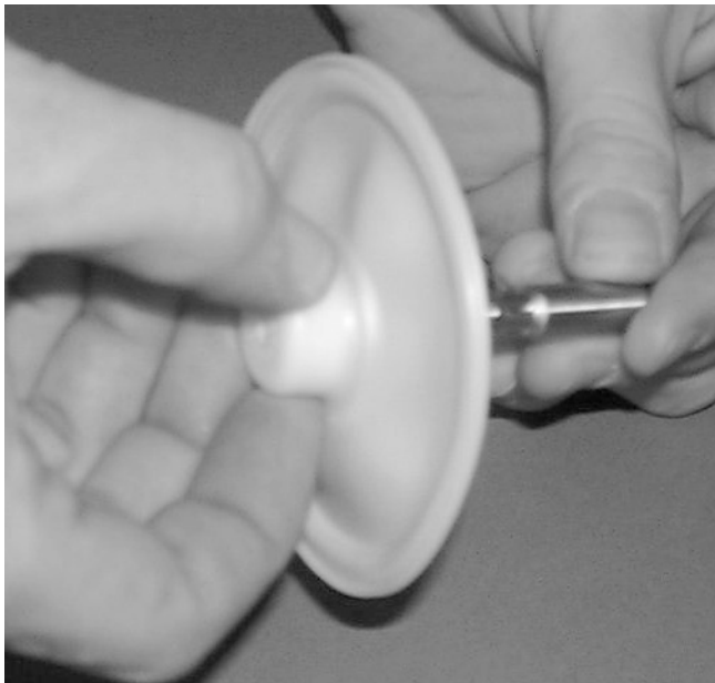
Step 10 For PTFE fitted pumps diaphragms, remove diaphragm by turning in a counter-clockwise direction.
