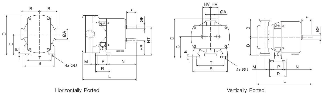
Horizontally Ported
