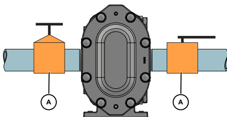
Figure 13 - Isolation Valves
