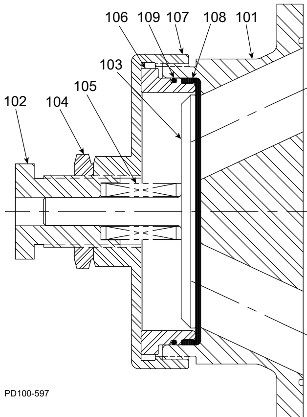
Figure 96 - Manual Vented Cover, 180-220-224 U2
