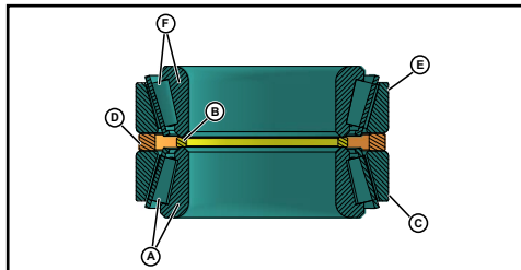
Figure 47 - Bearing assembly
