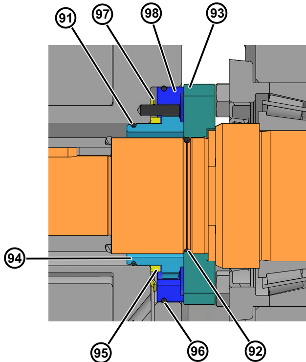
Figure 93 - High Pressure Barrier (HPB) Seal
