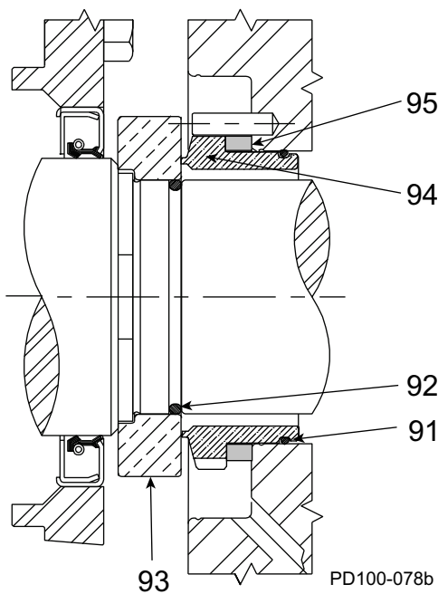
Figure 91 - NF Single Mechanical Seal
