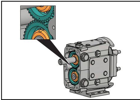
Figure 59 - Timing Gear Marks
