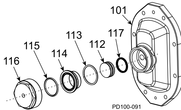
Figure 97 - Pneumatic Piston Vented Cover
