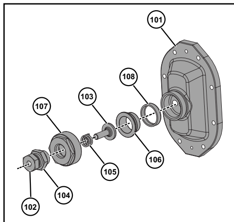
Figure 72 - Manual Cover
