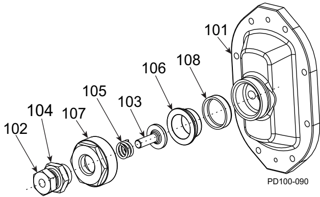
Figure 94 - Manual Vented Cover, 006-134-U2
