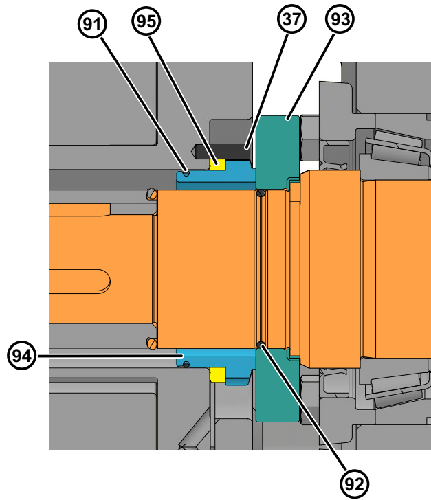
Figure 88 - Standard Single Mechanical Seal
