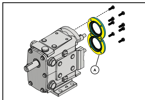
Figure 42 - Remove Sealant from Retainer
