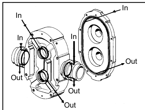
Figure 78 - Flushing Connection - Aseptic Series
