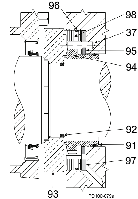
Figure 92 - NF Double Mechanical Seal
