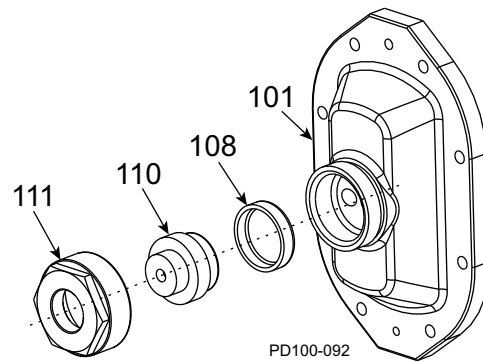
Figure 95 - Pneumatic Diaphragm Vented Cover
