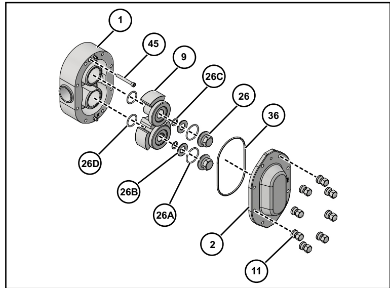
Figure 33 - Exploded View of Fluid Head
