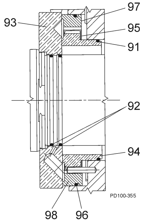
Figure 90 - Aseptic Design Double Mechanical Seal (213, 323 U2 ONLY)
