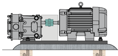
Figure 6 - Permanent Installation on Foundation
