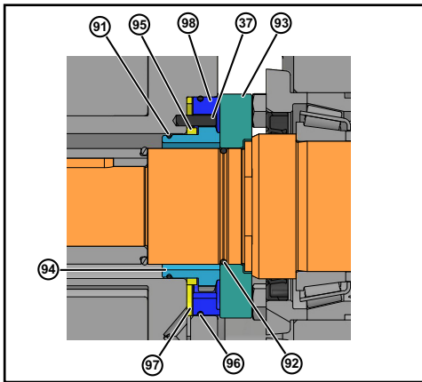
Figure 68 - Double Mechanical Seal
