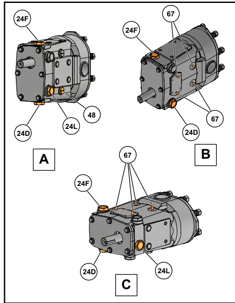
Figure 27 - Lubrication Points
