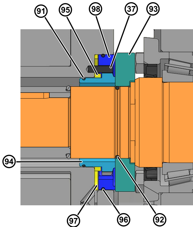
Figure 89 - Standard Double Mechanical Seal
